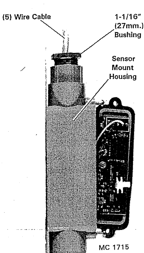
Figure 10 - Weather Sensor
