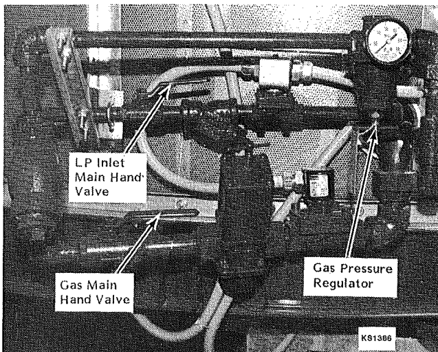
Figure 6 - LP Piping
