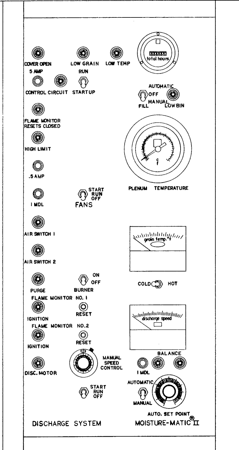
Figure 5 - Control Panel
