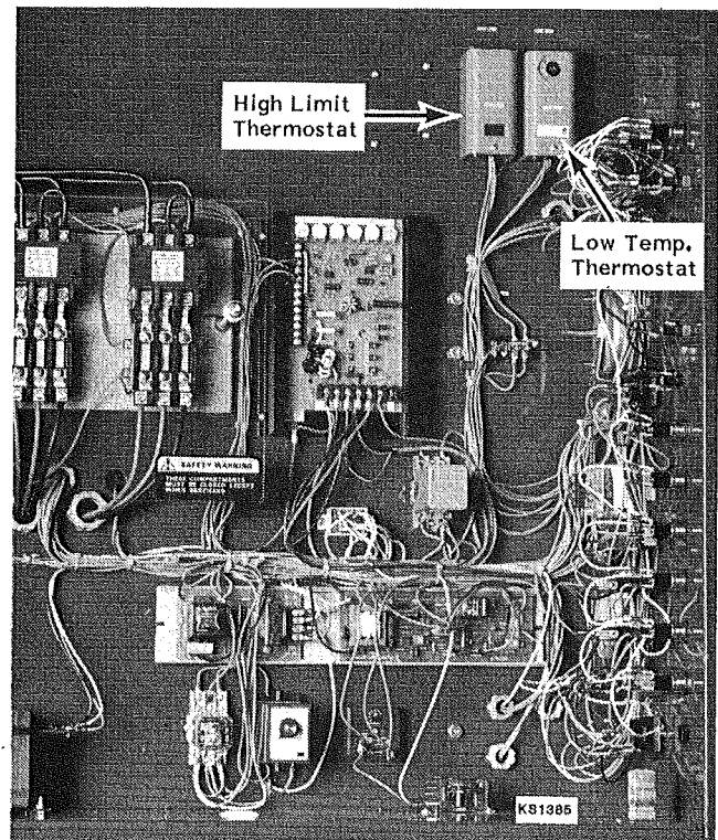
Figure 7 - High Limit and Low Temp. Thermostats
