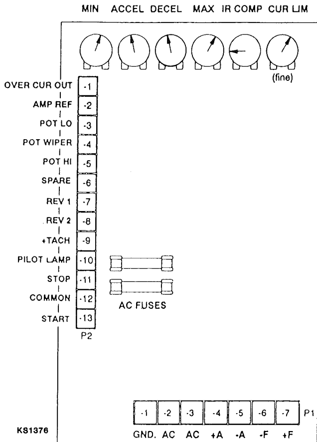
FIGURE 12 – 500 SERIES SCR BOARD
