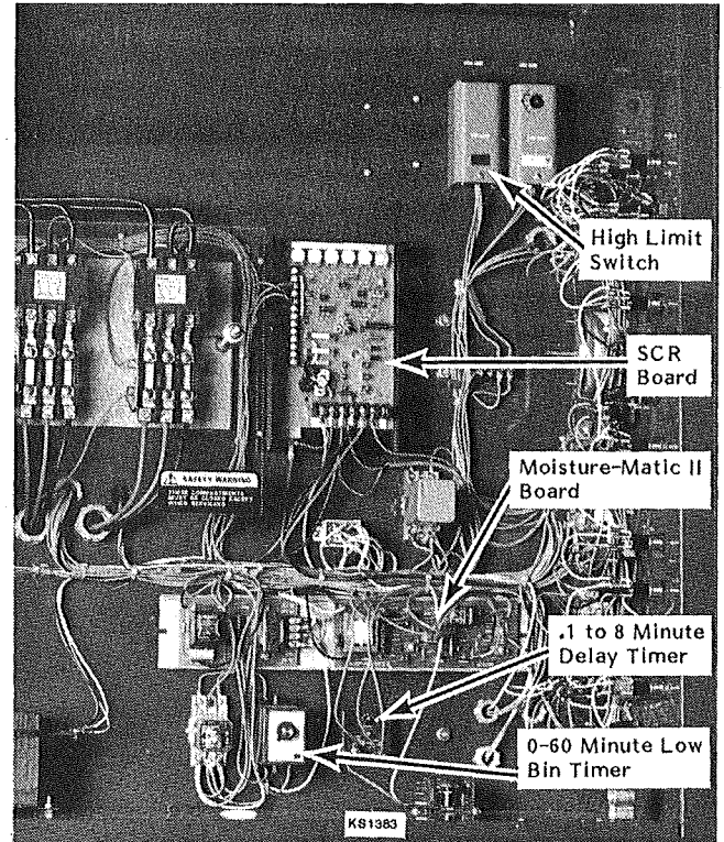
Figure 8 - Control Cabinet (Inside)
