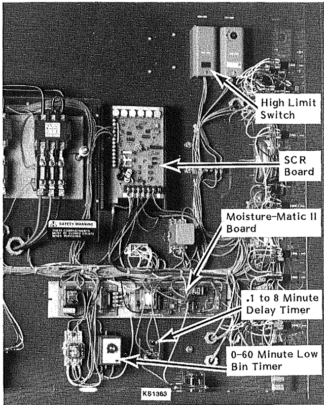
Figure 11 - Control Cabinet (Inside)
