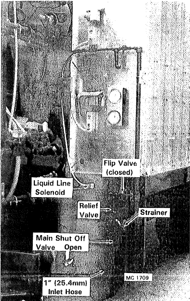
Figure 11 - Liquid Propane Supply Manifold
