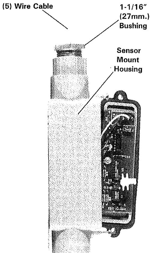
Figure 35 - Weather Sensor
