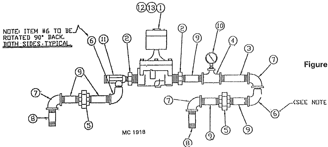
Figure 12 - Natural Gas Supply Manifold
