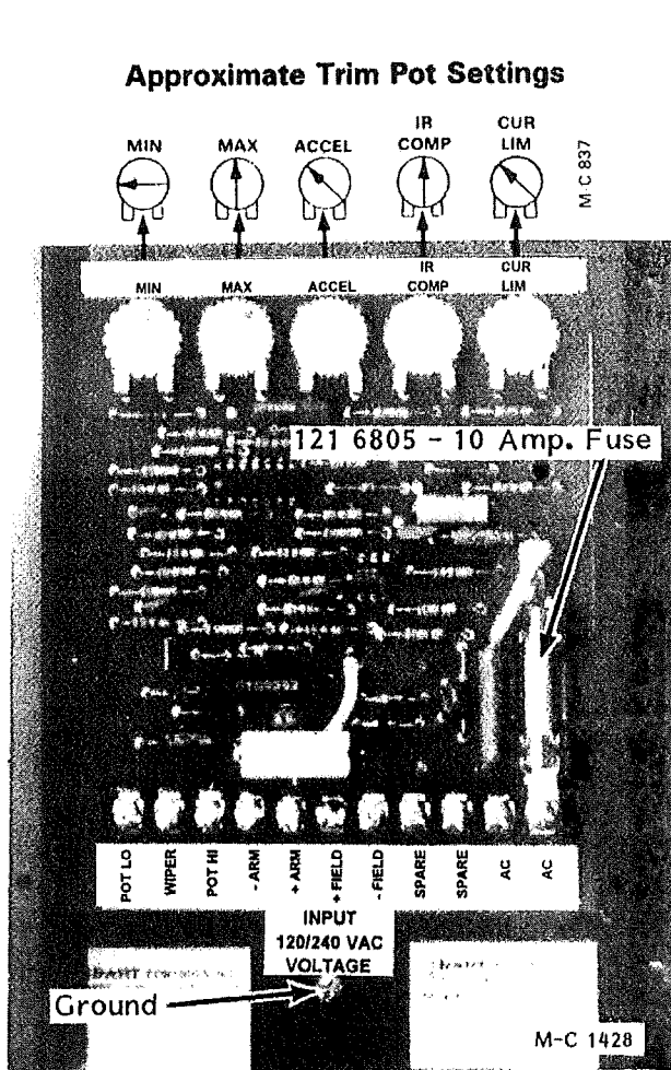
Figure 47 - SCR Drive Control Board
