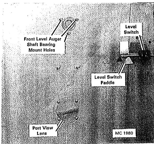
Figure 2 - Level Switch (Inside Hopper View - 410-820)
