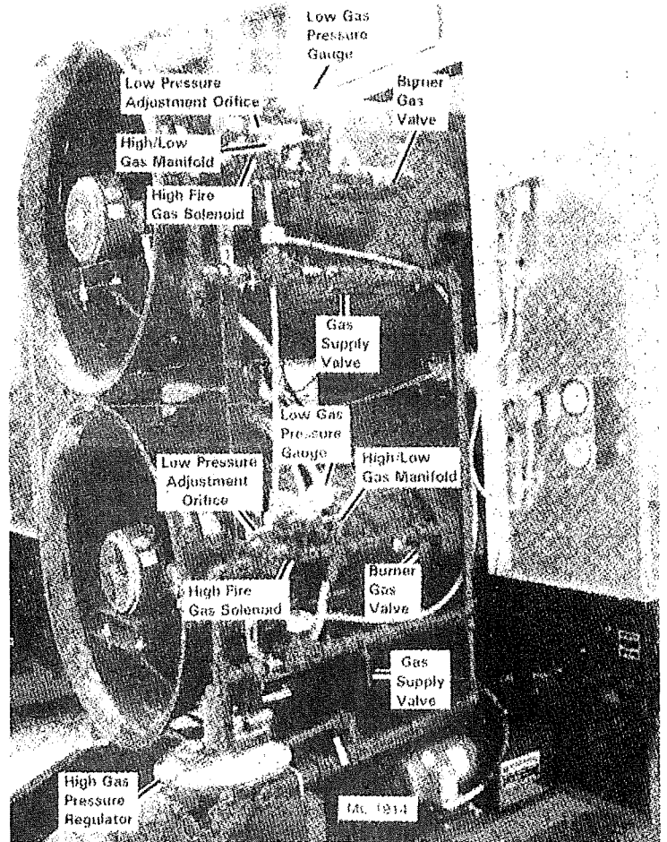
Figure 12 - Natural Gas Supply Manifold
