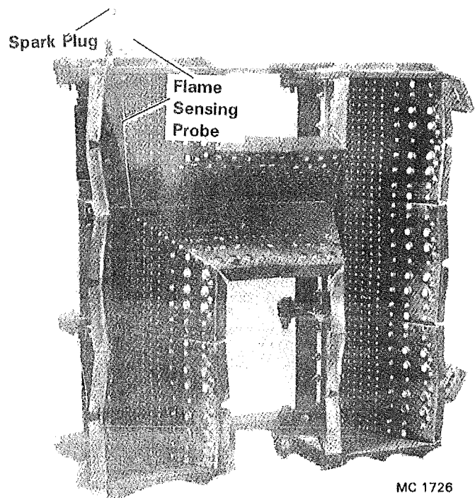
Figure 45 - 4 MBTU Burner - 720/820 Bottom
