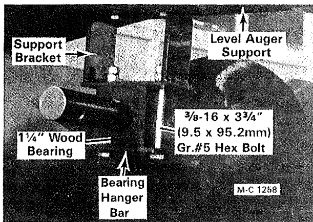
Figure 3 - Level Auger Bearing
