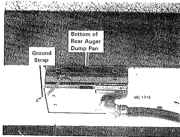
Moisture Monitor Sensor Installation
