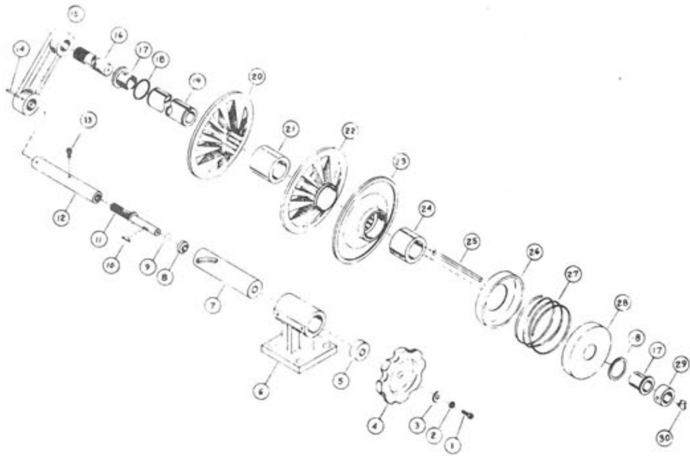
VARIABLE PULLEY ASSEMBLY No. 4430
